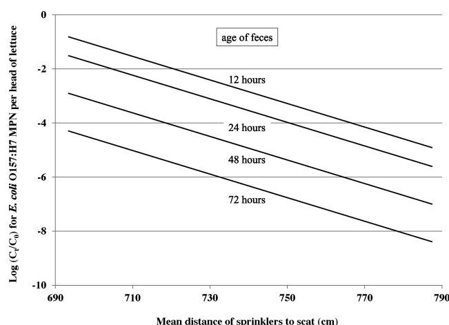
FIGURE 3. Model 2: predicted concentration of E. coli O157:H7 per head of romaine lettuce on the windward (north-northwest facing) side of the bed as a function of age of feces and distance to sprinklers, based on data from the high concentration assay.
