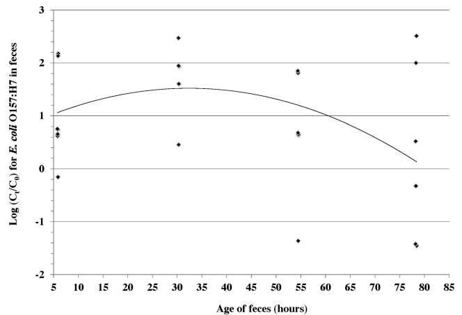
FIGURE 4. Effect of age of feces on amount of E. coli O157:H7 per fecal deposit remaining after irrigation ( C_t ), relative to initial load ( C_0 = 1.29 \times 10^8 CFU per fecal deposit).
