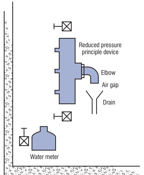
FIGURE 35. Typical installation reduced pressure principle device vertical illustration.
