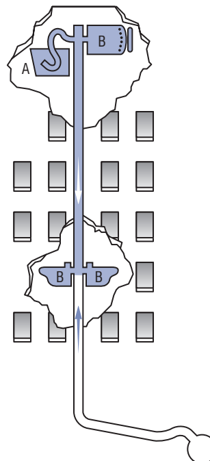
FIGURE 44. Backsiphonage (Case 1).
