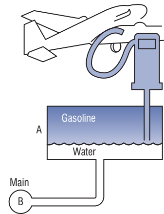
FIGURE 48. Backsiphonage (Case 5).
