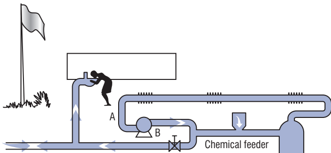
FIGURE 50. Backflow (Case 1).
