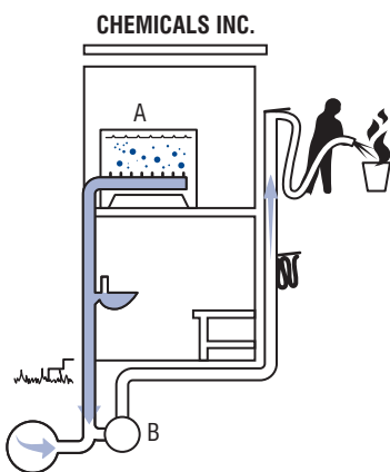
FIGURE 46. Backsiphonage (Case 3).
