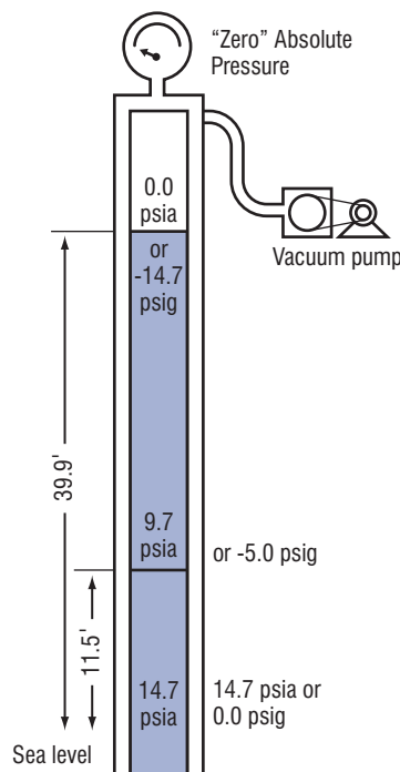
FIGURE 4. Effect of evacuating air from a column.
