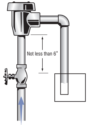
FIGURE 16. Atmospheric vacuum breaker typical installation.
