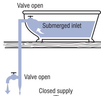
FIGURE 7. Backsiphonage in a plumbing system.
