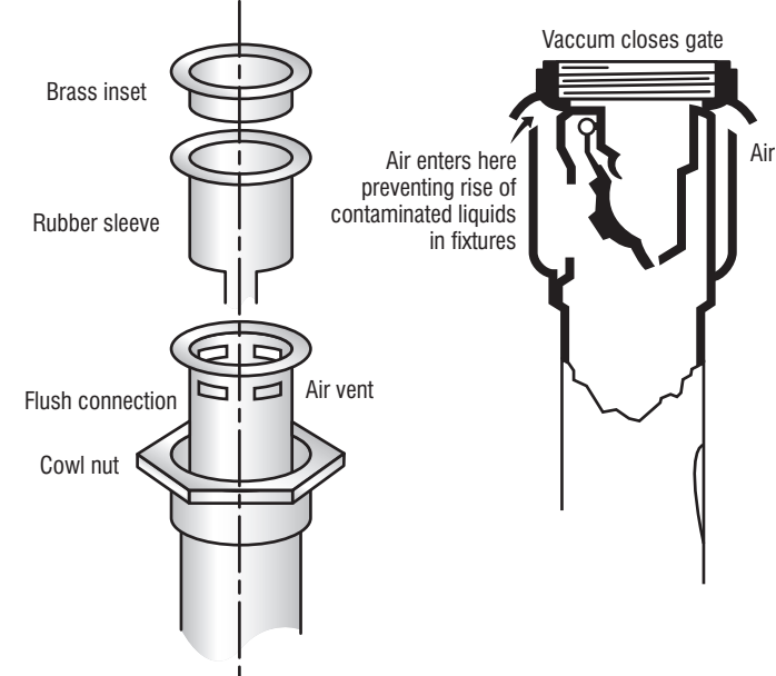
FIGURE 57. Vacuum breakers.
